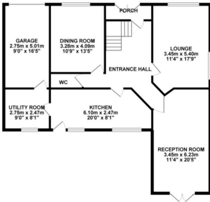
GROUND FLOOR 104.88 sq. m. ( 1128.88 sq. ft. )
